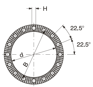
Hirth Serrations
