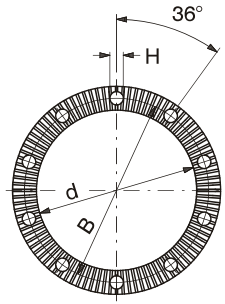
Hirth Serrations
